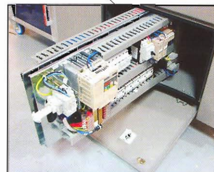
Control Panel slides out for easy access to all electrical components.
